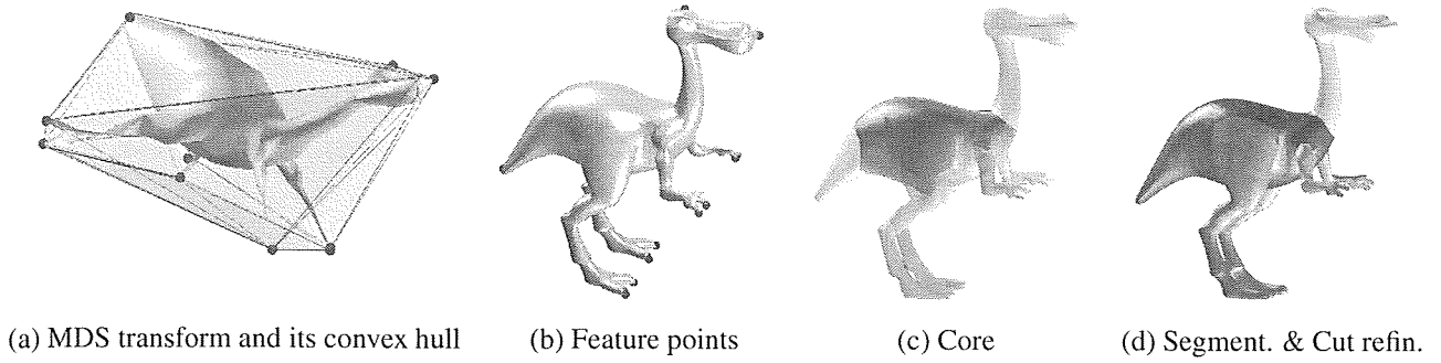
Figure 2. Algorithm [14] outline.
