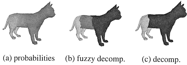
Figure 1. Algorithm [15] outline.
